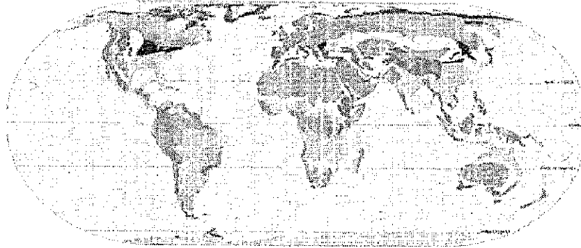
Climatic Zones BASED ON KÖPPEN SYSTEM
